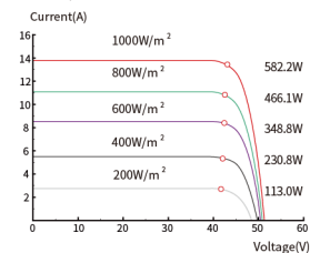
Current-Voltage Curve (580W) Cells temp.=25°C
