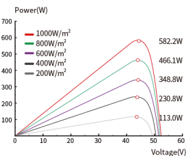
Power-Voltage Curve (580W) Cells temp.=25°C
